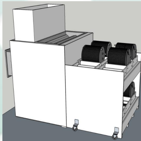
Open drum dryer
