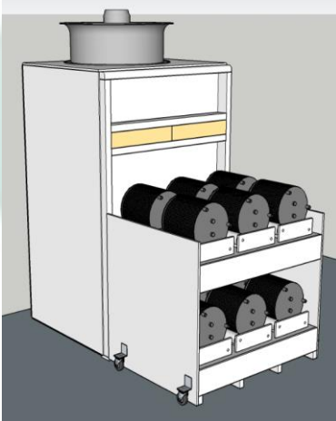
Box drying installation
