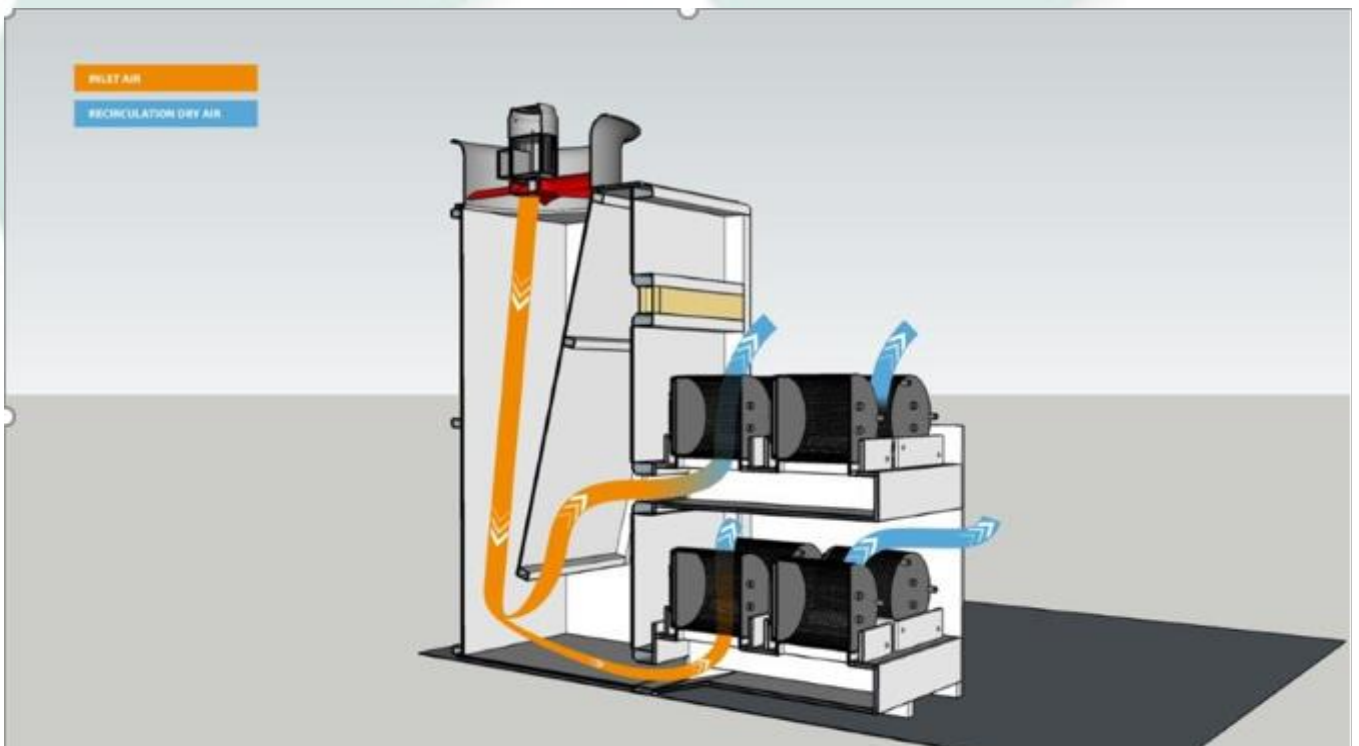
Airflow is controlled by the box drying installation.
